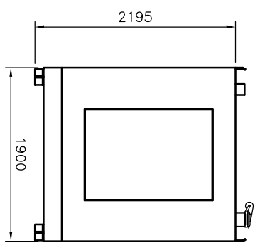
VISTA LATO MARMITTE SILENCER SIDE VIEW
